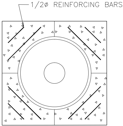
REINFORCING DETAIL SECTION "A-A"
